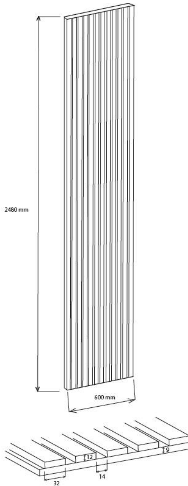
Figure 2 Drawing of Acupanel FR-panels.
